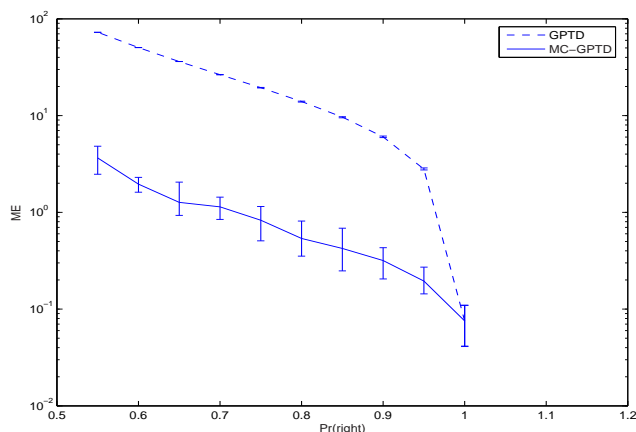
Figure 2. MC-GPTD compared with the original GPTD on the random-walk MDP. The mean error after 400 episodes for each algorithm is plotted against \text{Pr}(\text{right}) .
