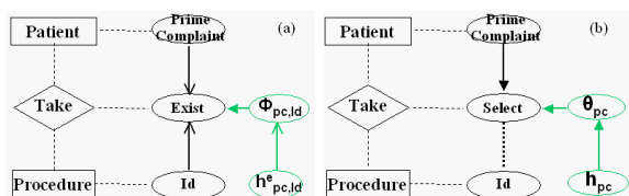
Figure 2. DAPER models with structure uncertainty over medical domain, which is modelled using the formalism of Getoor et al. (2003). (a)existence uncertainty modelling. (b)reference uncertainty modelling. The attribute Take.Select is modelled as a multinomial variable with as many states as there are procedures. \theta_{s|pc} is the parameter vector for the multinomial distribution and h_{pc} are the parameters of the prior distribution.
